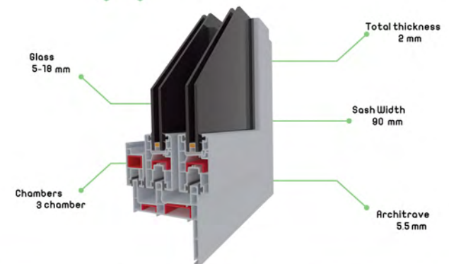
Sliding S100 mm
